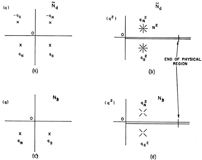
FIG. 3. The positions of the singularities of \tilde{N}_d and N_\delta . (a) Singularities of \tilde{N}_d in the q plane; (b) singularities of \tilde{N}_d in the q^2 plane; (c) singularities of N_\delta in the q plane; (d) singularities of N_\delta in the q^2 plane. In the q^2 ( s ) planes, broken diagonal crosses refer to the second sheet in s , \text{Im}q < 0 . Note that q_S^* = -q_N , and q_N^* = -q_S .
